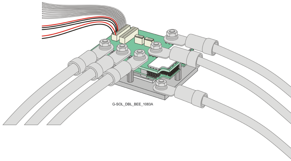
Figure 16: Connecting the Feedback Wires
