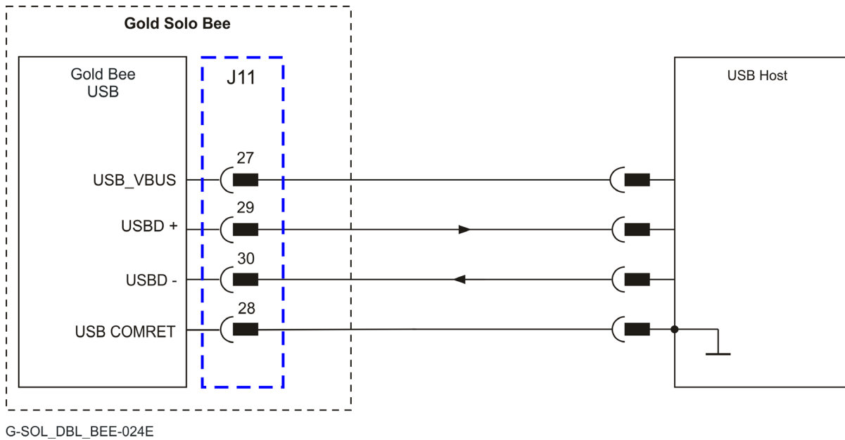
Figure 43: USB Network Diagram
