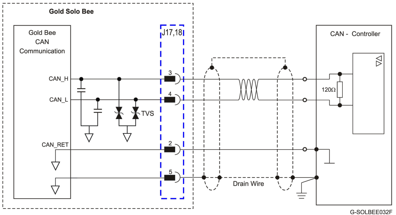
Figure 47: CAN Interface
