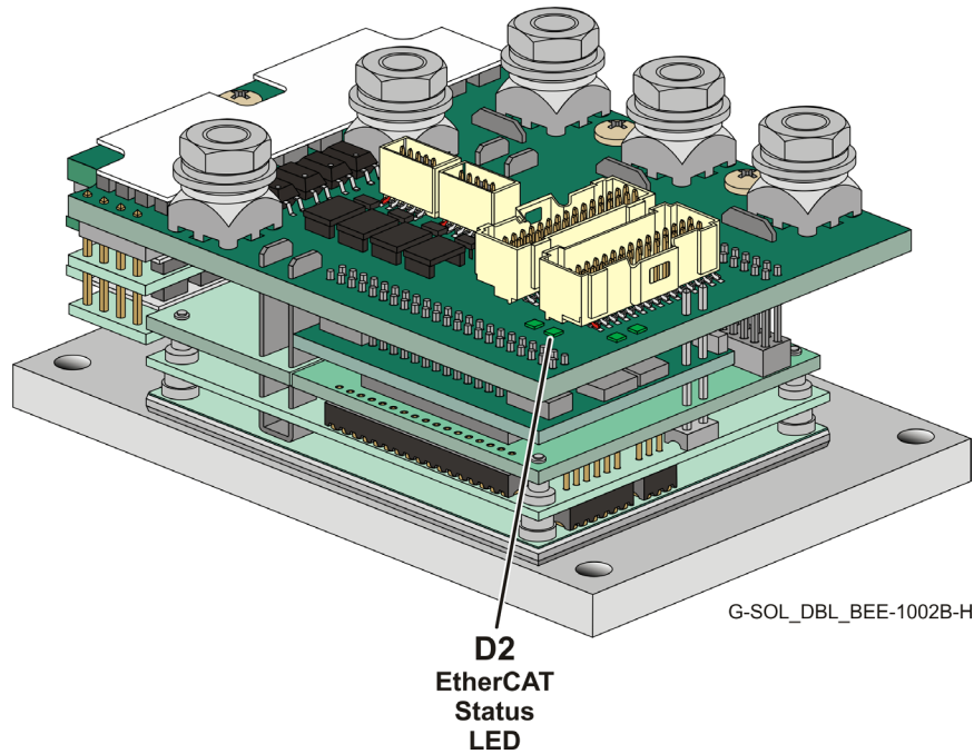
Figure 45: EtherCAT Status LED
