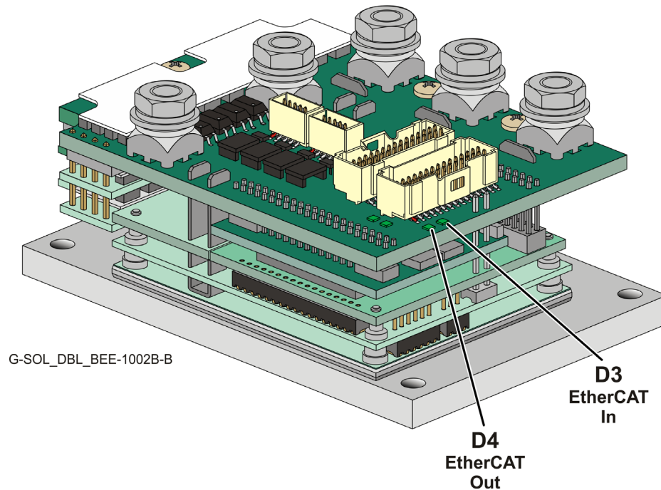
Figure 46: Ethernet Connector LEDs
