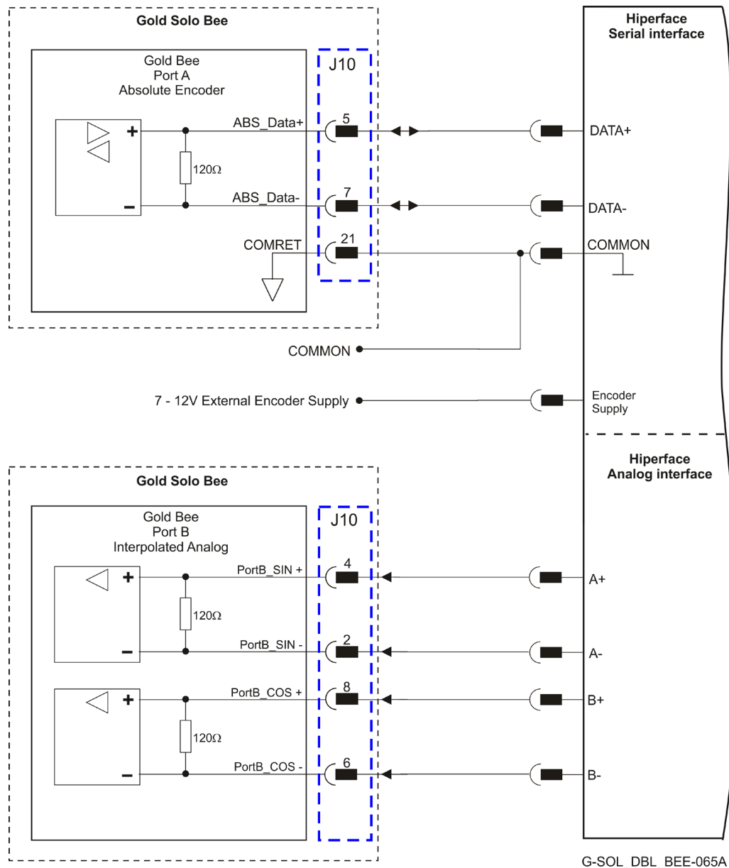
Figure 20: Absolute Serial Encoder – Recommended Connection Diagram for Stegmann Hiperface
