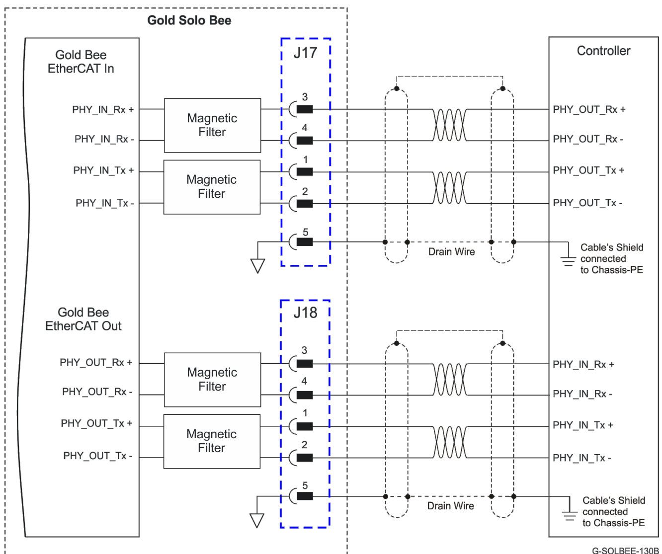
Figure 44: EtherCAT Connection Schematic Diagram
