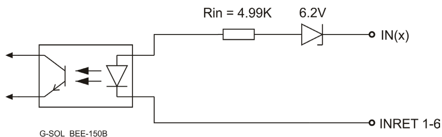
Figure 27: Digital Input PLC Source Schematic
