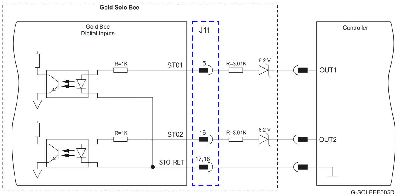
Figure 40: STO Input Connection – PLC (24V Logic)
