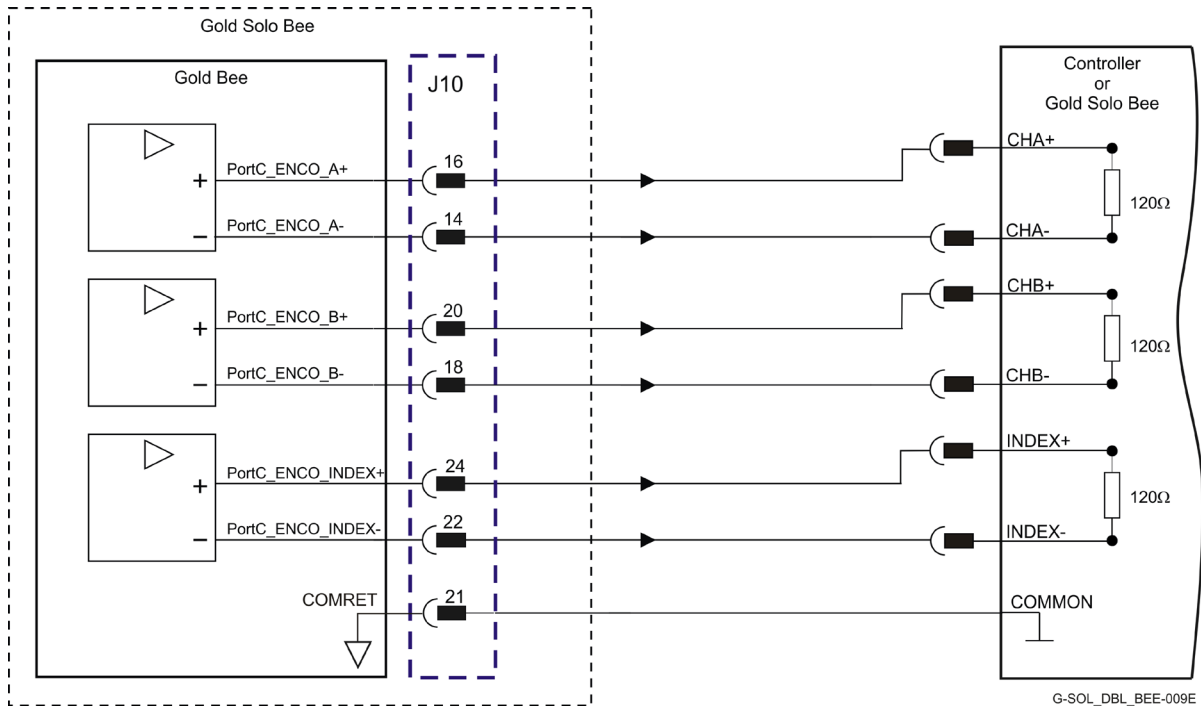
Figure 25: Emulated Encoder Differential Output – Recommended Connection Diagram
