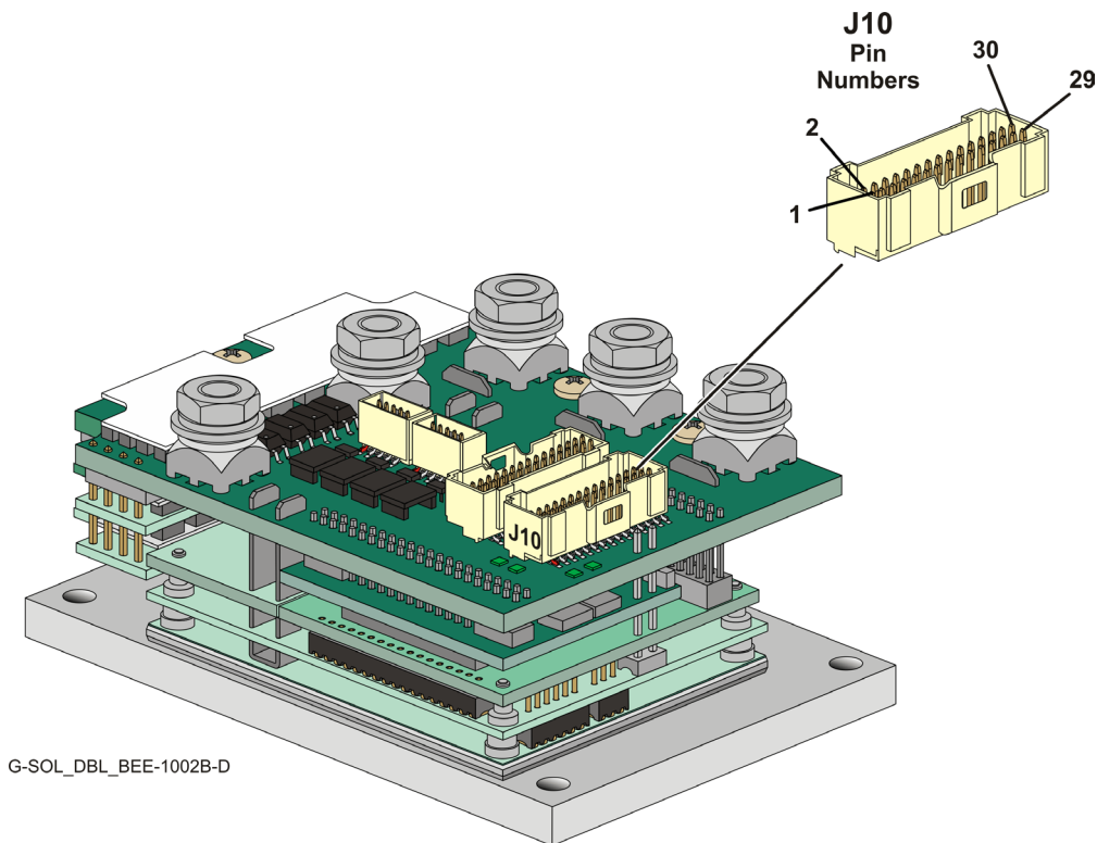
J10 VL & Feedback Connector
