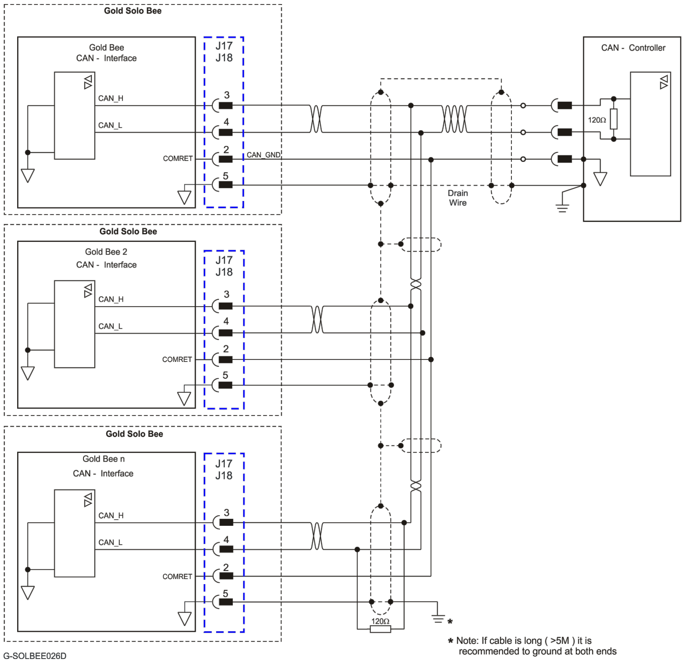
Figure 48: CAN Network Diagram – Drop Off Topology
