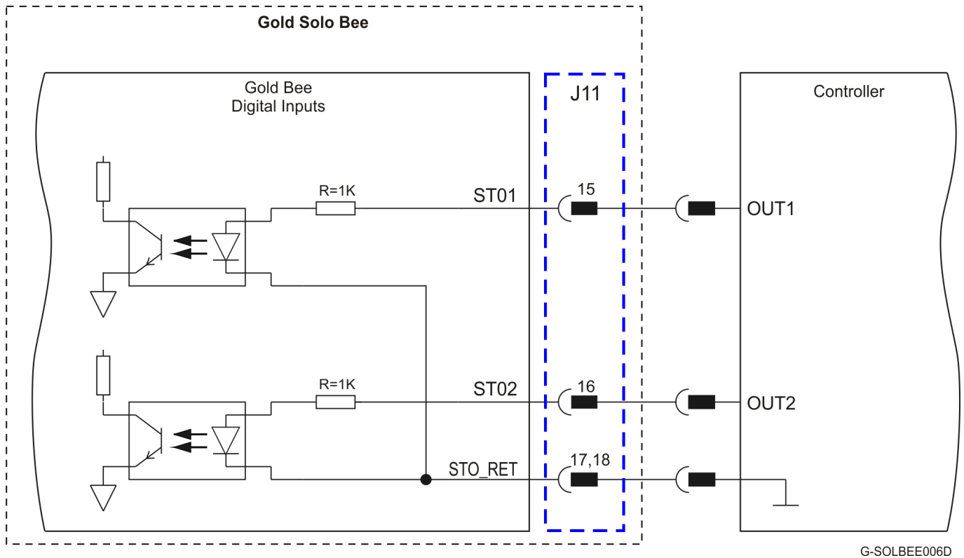
Figure 39: STO Input Connection – 5V Logic
