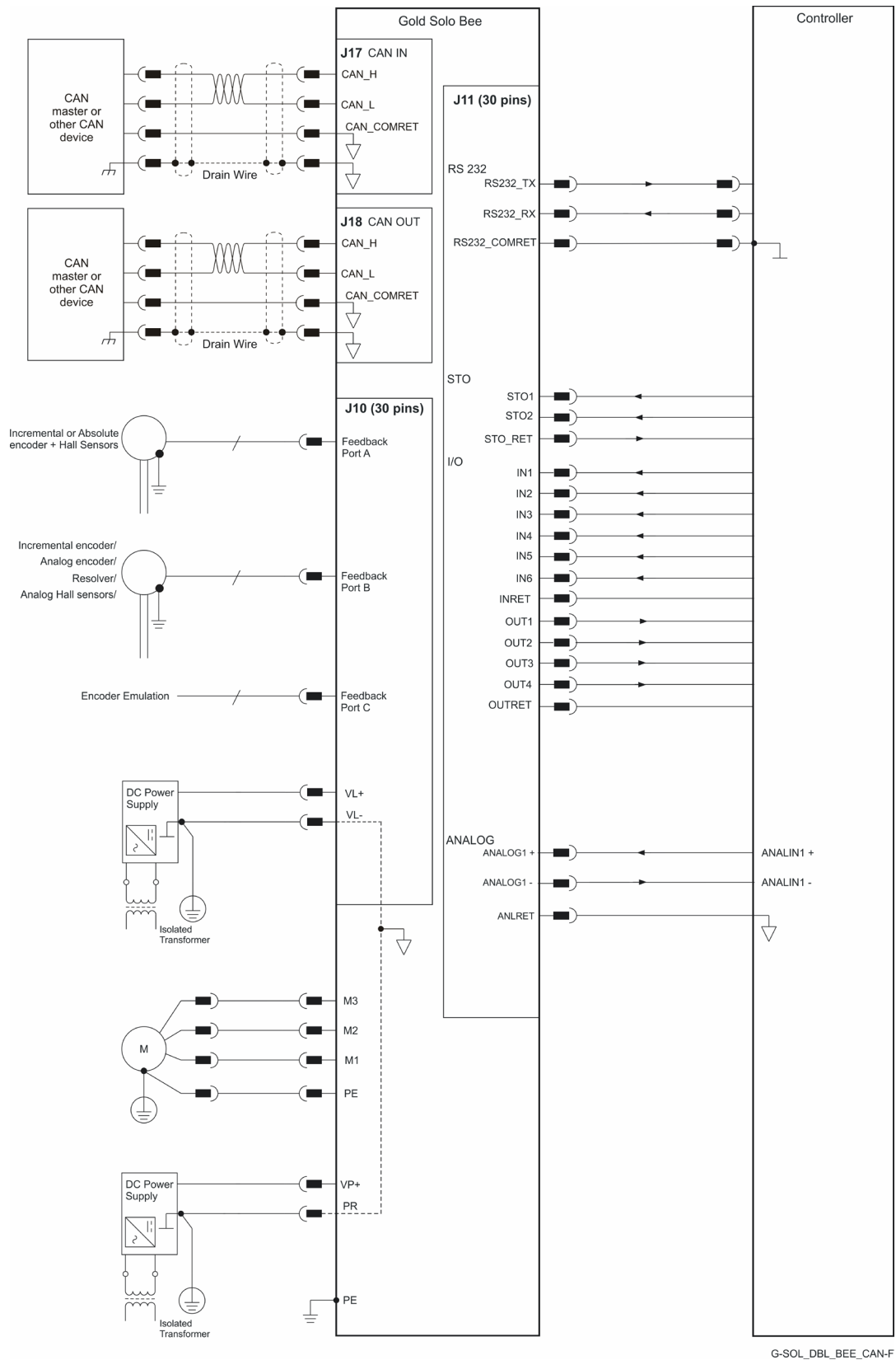
Figure 3: The Gold Solo Double Bee CAN Connection Diagram
