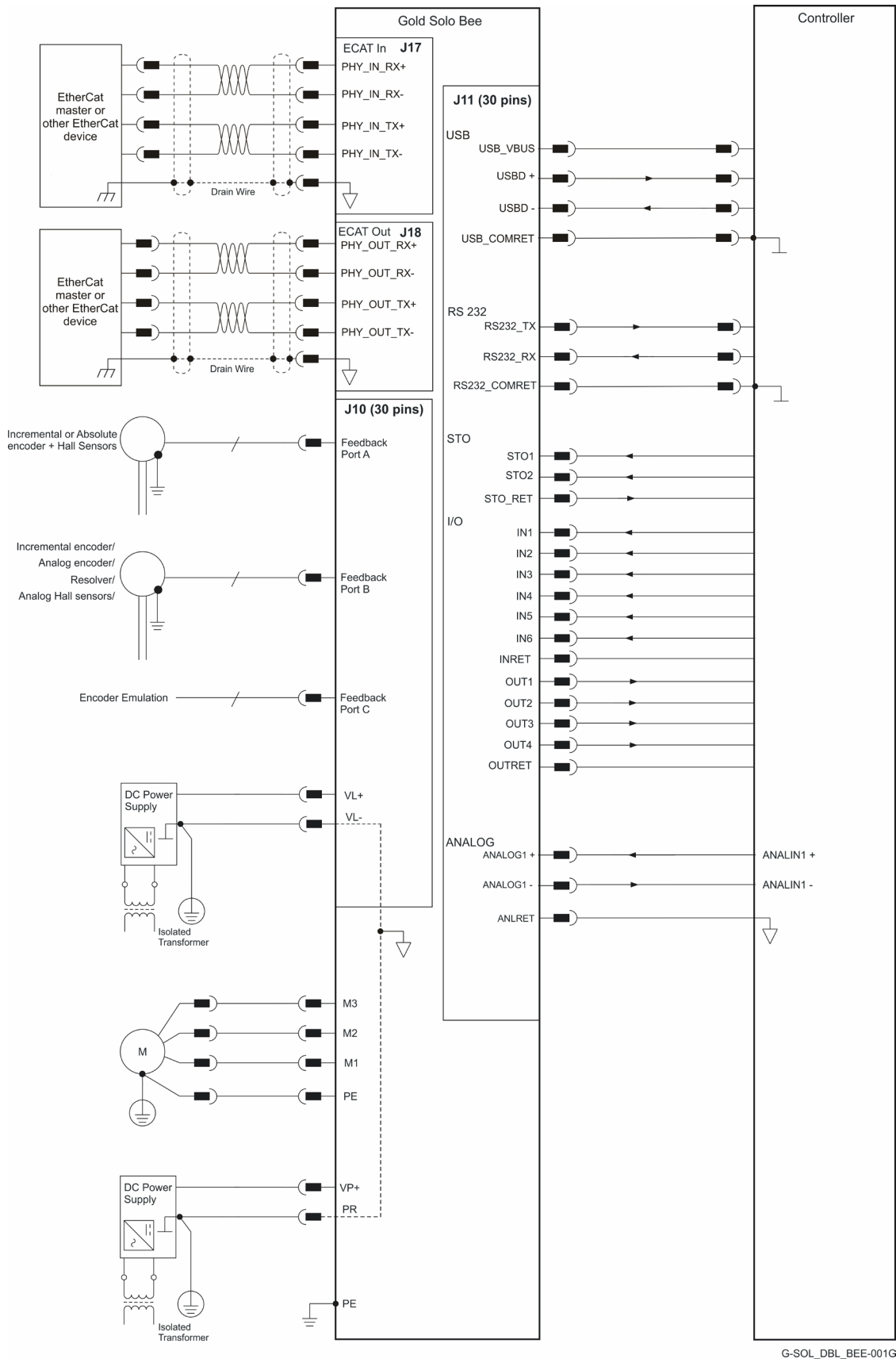
Figure 4: The Gold Solo Double Bee EtherCAT Connection Diagram
