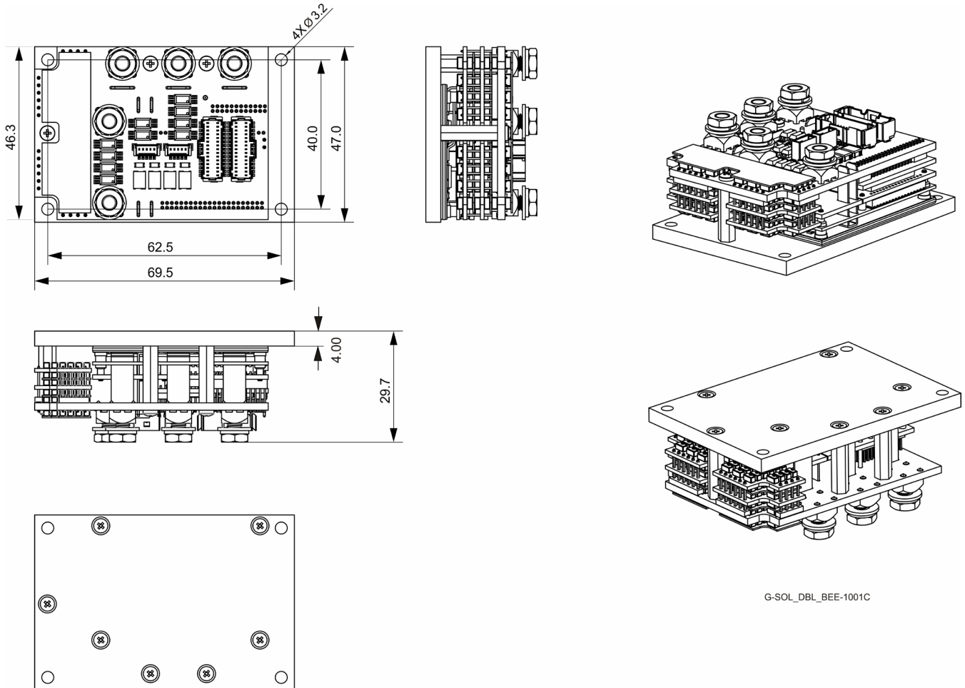
Figure 49: G-Solo Double Bee –EtherCAT version
