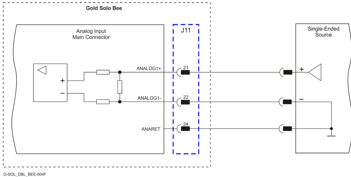
Figure 41: Analog Input
