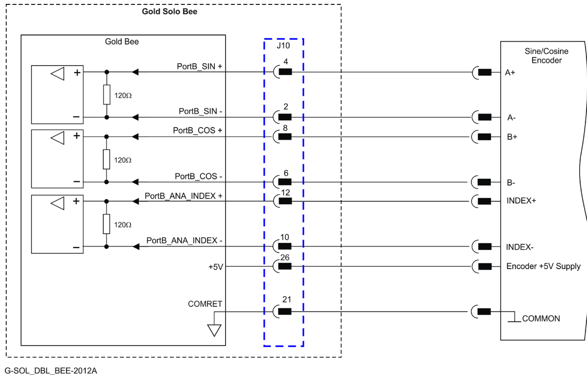
Figure 23: Port B - Interpolated Analog Encoder Connection Diagram
