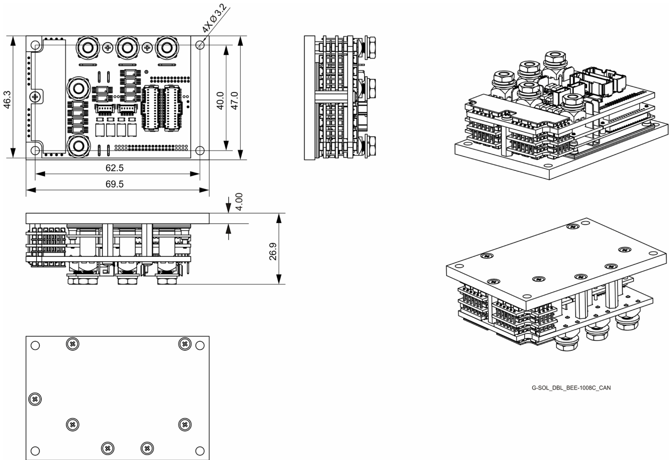
Figure 50: G-Solo Double Bee –CAN version
