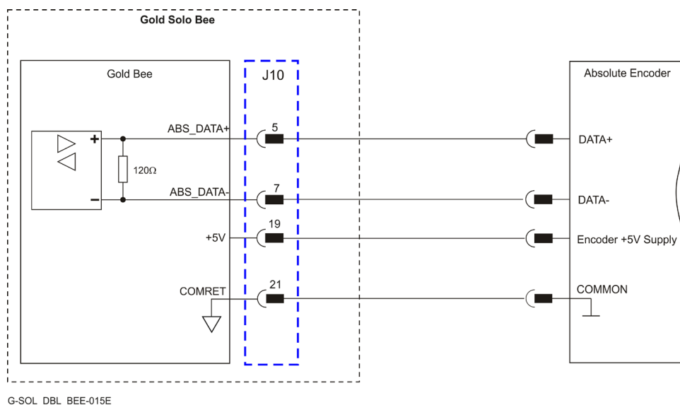
Figure 19: Absolute Serial Encoder – Recommended Connection Diagram for Sensors Supporting Data Line Only (NRZ types, e.g., Panasonic / Mitutoyo / etc.)
