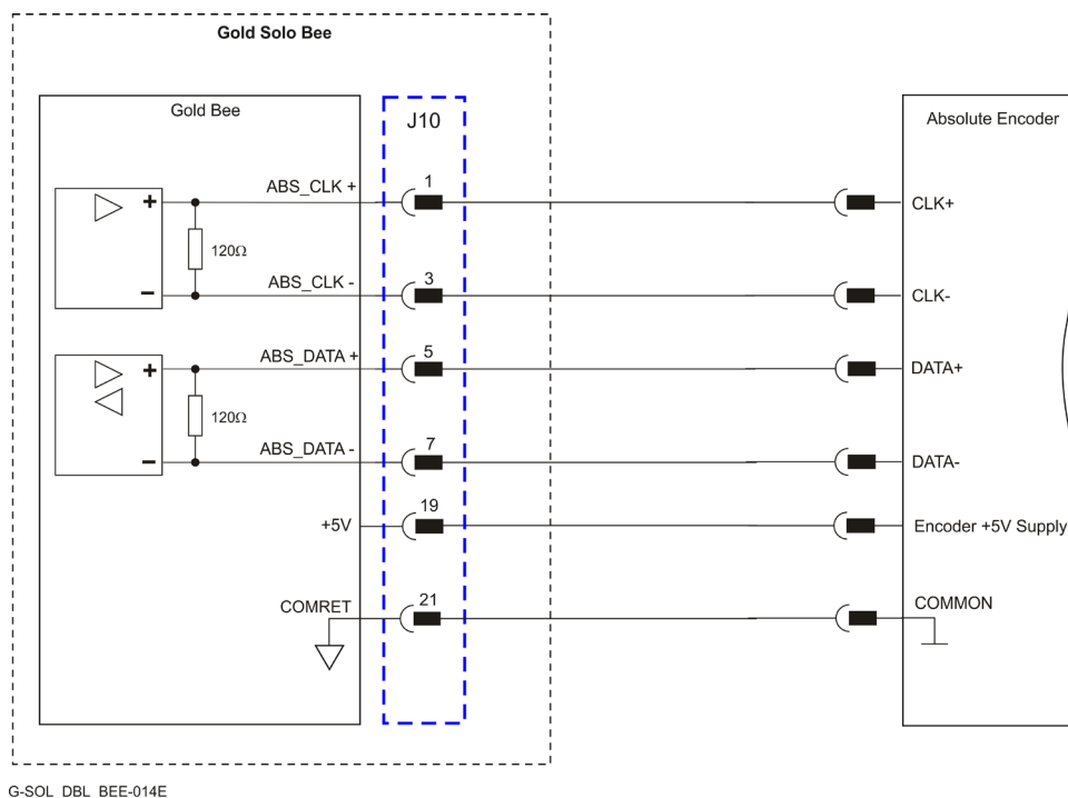
Figure 18: Absolute Serial Encoder – Recommended Connection Diagram for Sensors Supporting Data/Clock (e.g., Biss / SSI / EnDAT, etc.)
