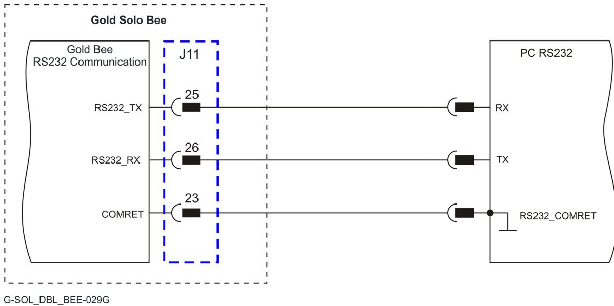
Figure 42: Standard RS-232 Connection Diagram
