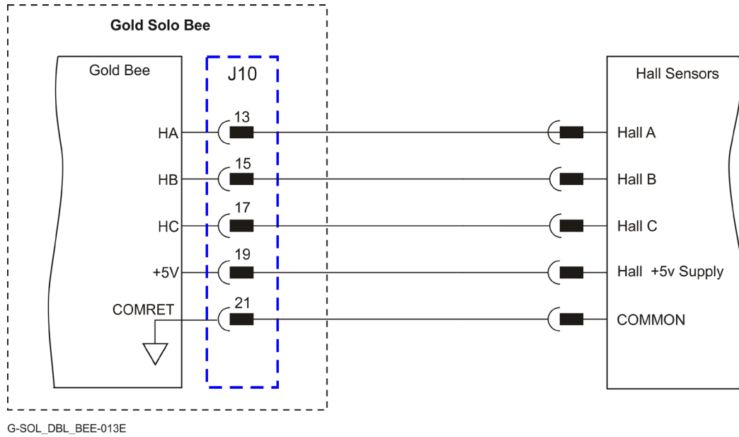
Figure 21: Hall Sensors Connection Diagram
