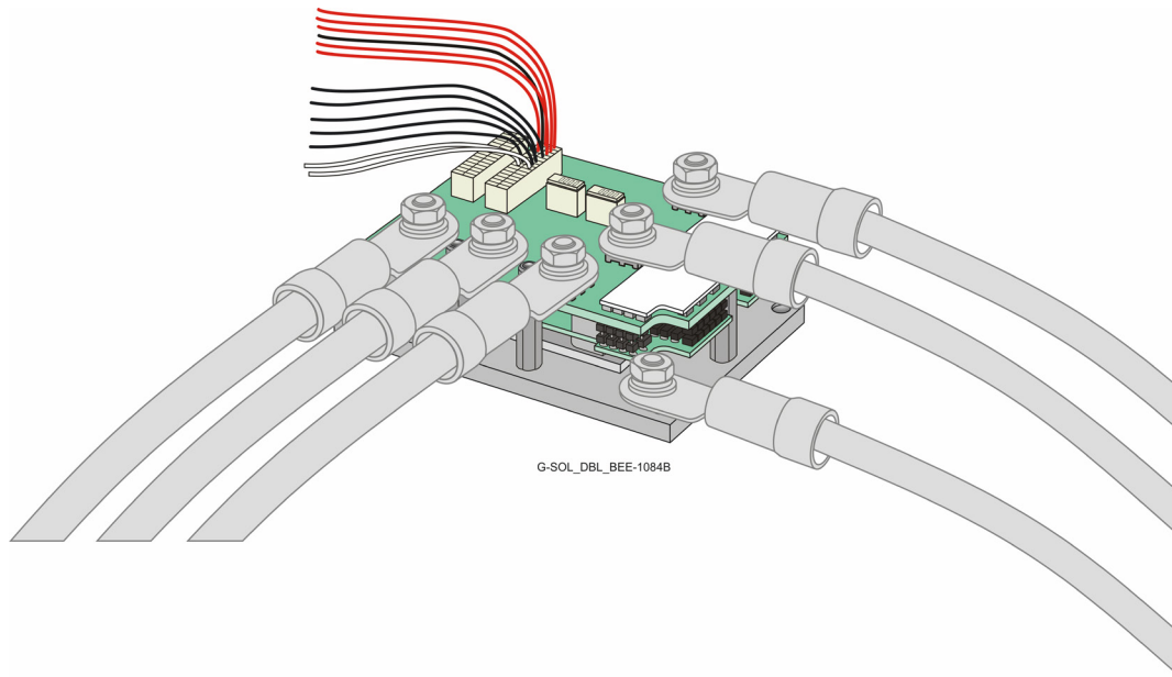
Figure 26: Connecting the USB, RS232, and Analog Input Wires
