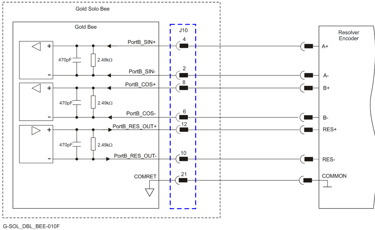
Figure 24: Port B – Resolver Connection Diagram
