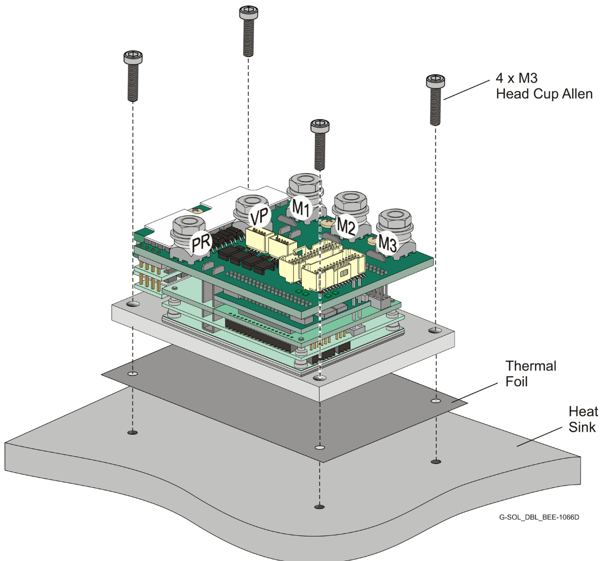
Figure 2: Mount the Heatsink and Thermal Foil to the Gold Solo Double Bee
