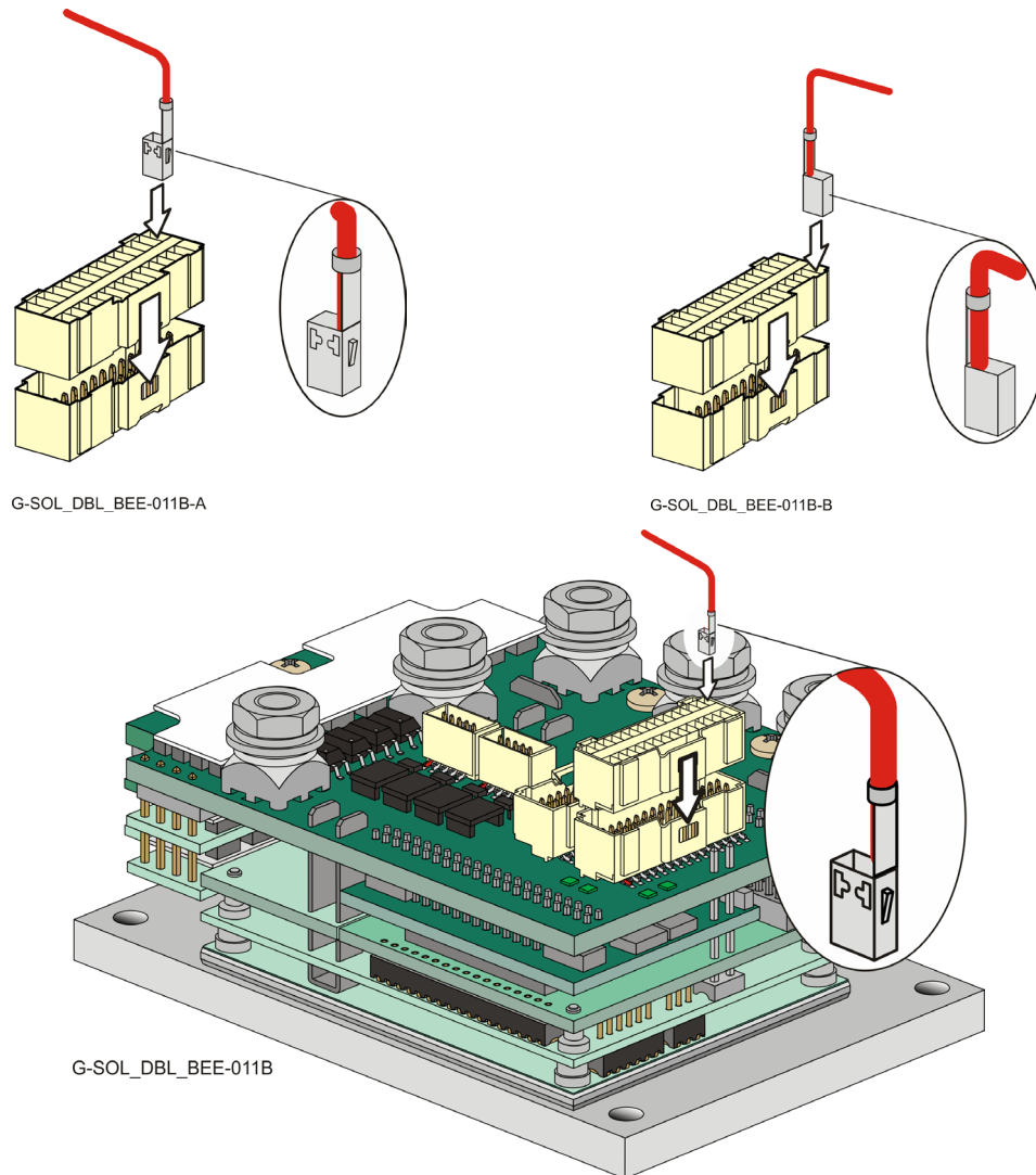
Figure 6: Inserting a wire/pin to the Female Connector
