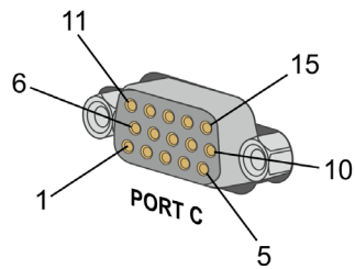
15-Socket High Density D-Type Connector
