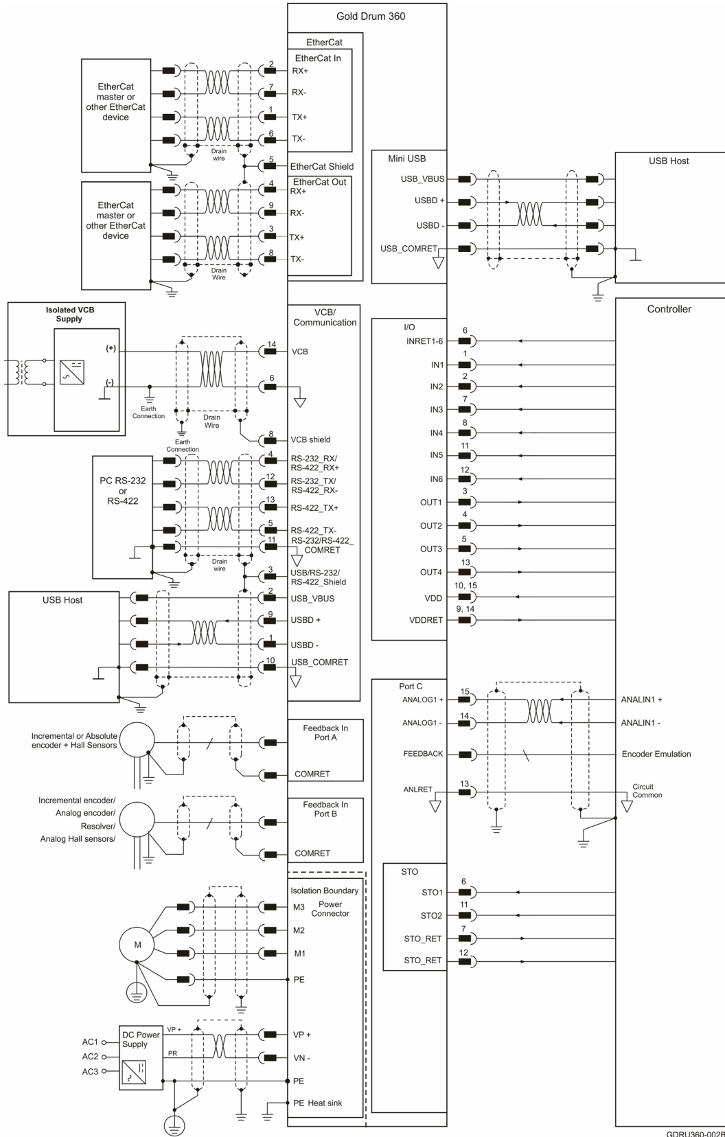
Figure 2: Gold Drum 360/430 Connection Diagram for EtherCAT
