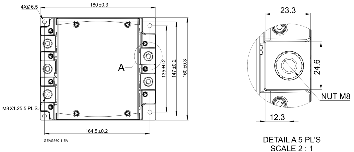
Figure 1: Mounting the Gold Drum 360/430
