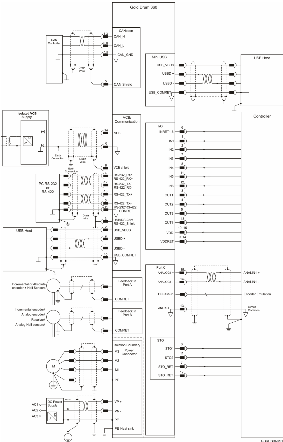
Figure 3: Gold Drum 360/430 Connection Diagram for CAN
