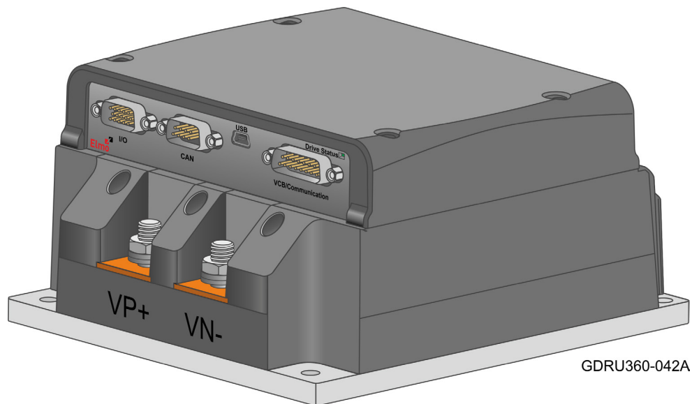
Figure 40: Drive Status Indicator LEDs on Gold Drum 360/430 – CAN Version
