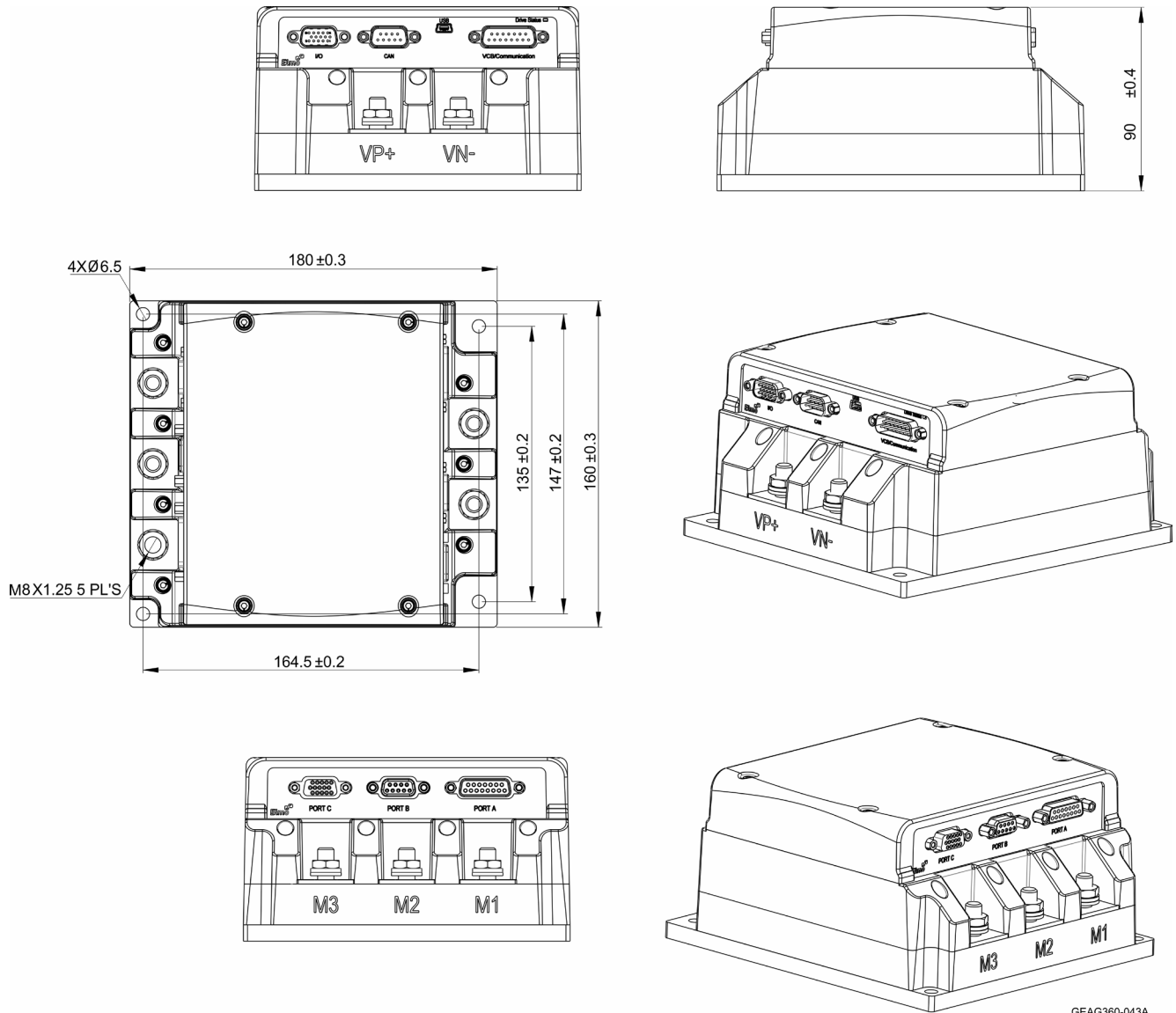
Figure 47: Gold Drum 360/430 CAN Version Dimensions
