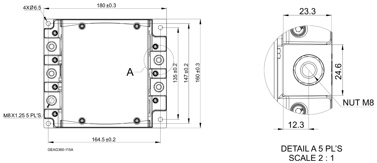
Figure 49: Gold Drum 360/430 Terminal Connectors' Dimensions
