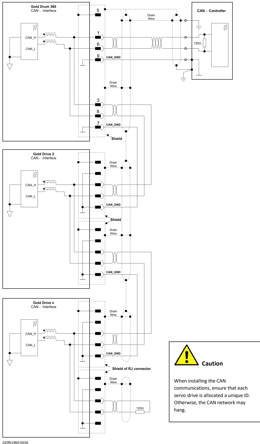
Figure 39: Gold Drum 360/430 Connection Diagram – CAN
