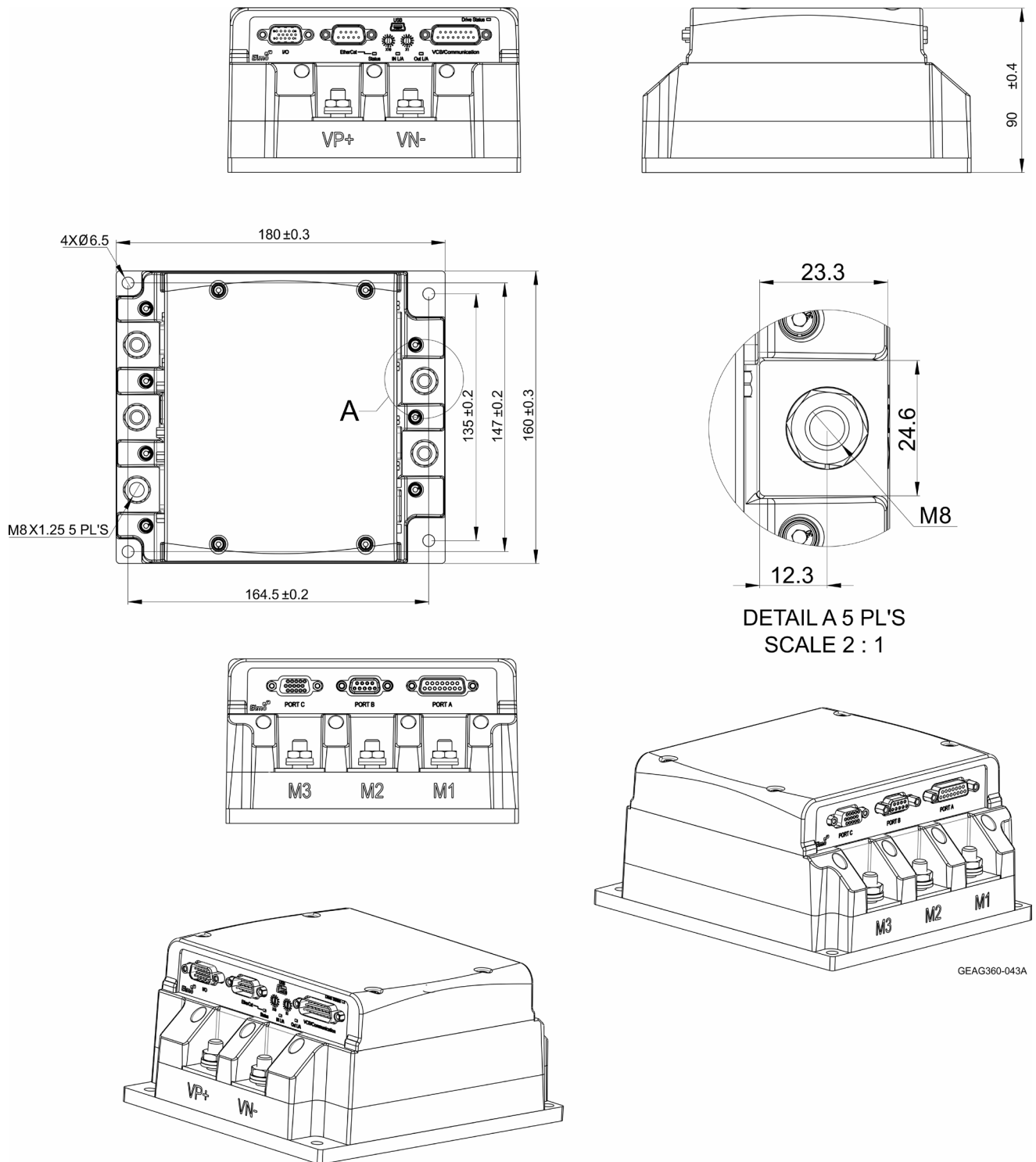
Figure 48: Gold Drum 360/430 EtherCAT Version Dimensions
