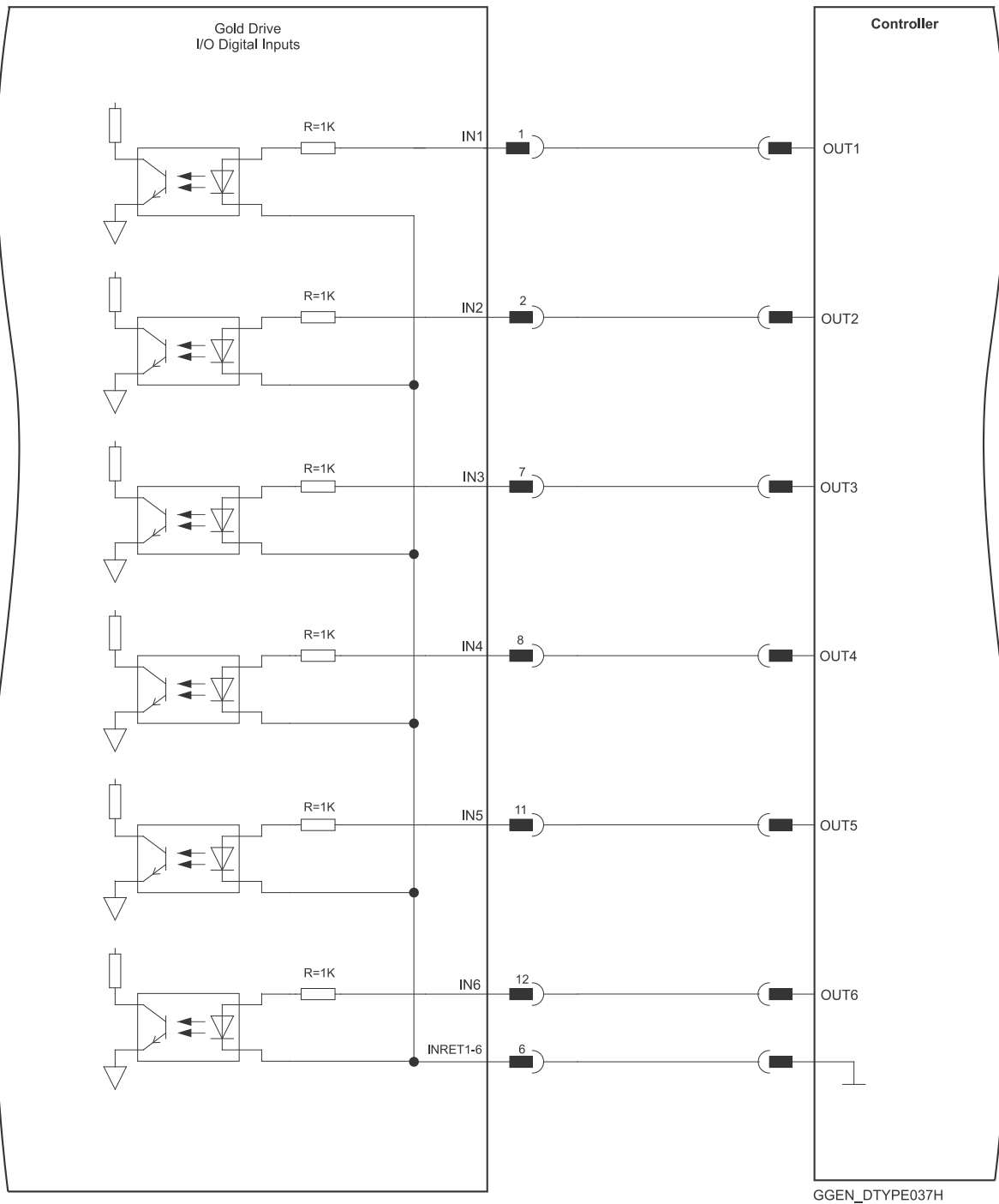
Figure 29: Digital Input TTL Mode D-Type Connection Diagram
