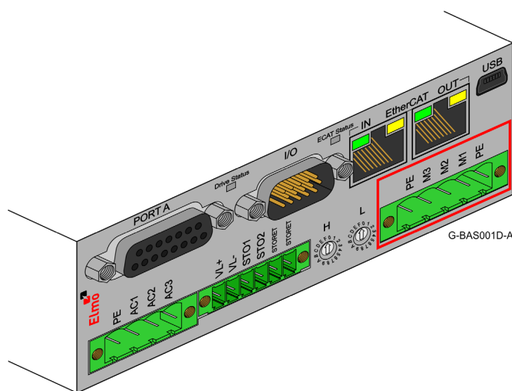
5-Pin Pluggable 5 mm Phoenix Screw Flange Connector
