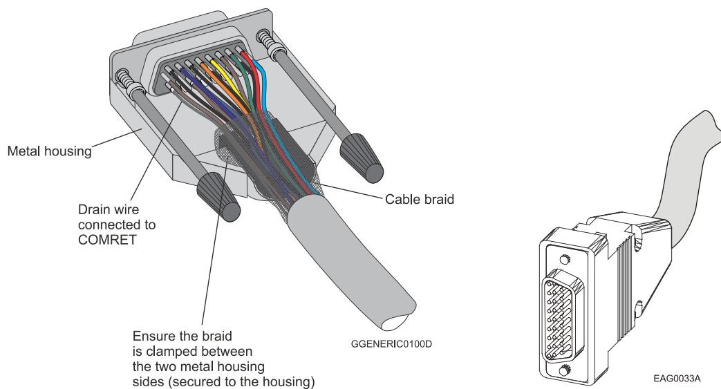
Figure 5: D-Type Cable Assemblies
