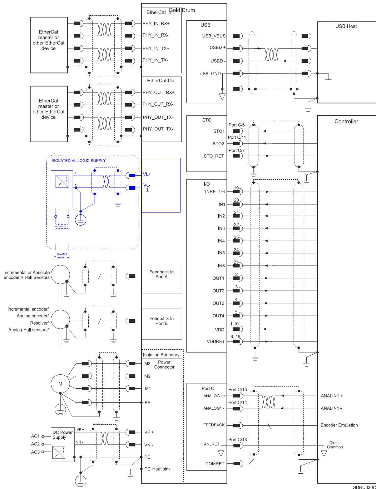
Figure 2: Gold Drum Connection Diagram - EtherCAT
