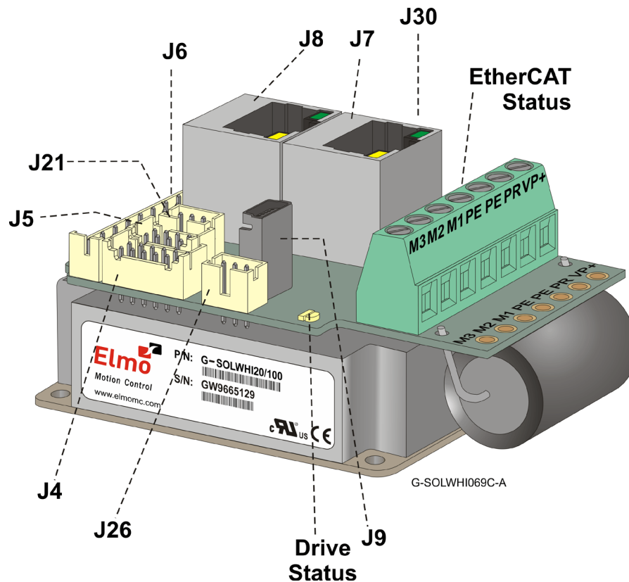
Figure 1: Connector Locations – EtherCAT
