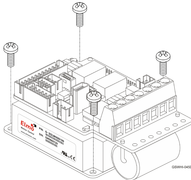
Figure 3: Mounting the Gold Solo Whistle
