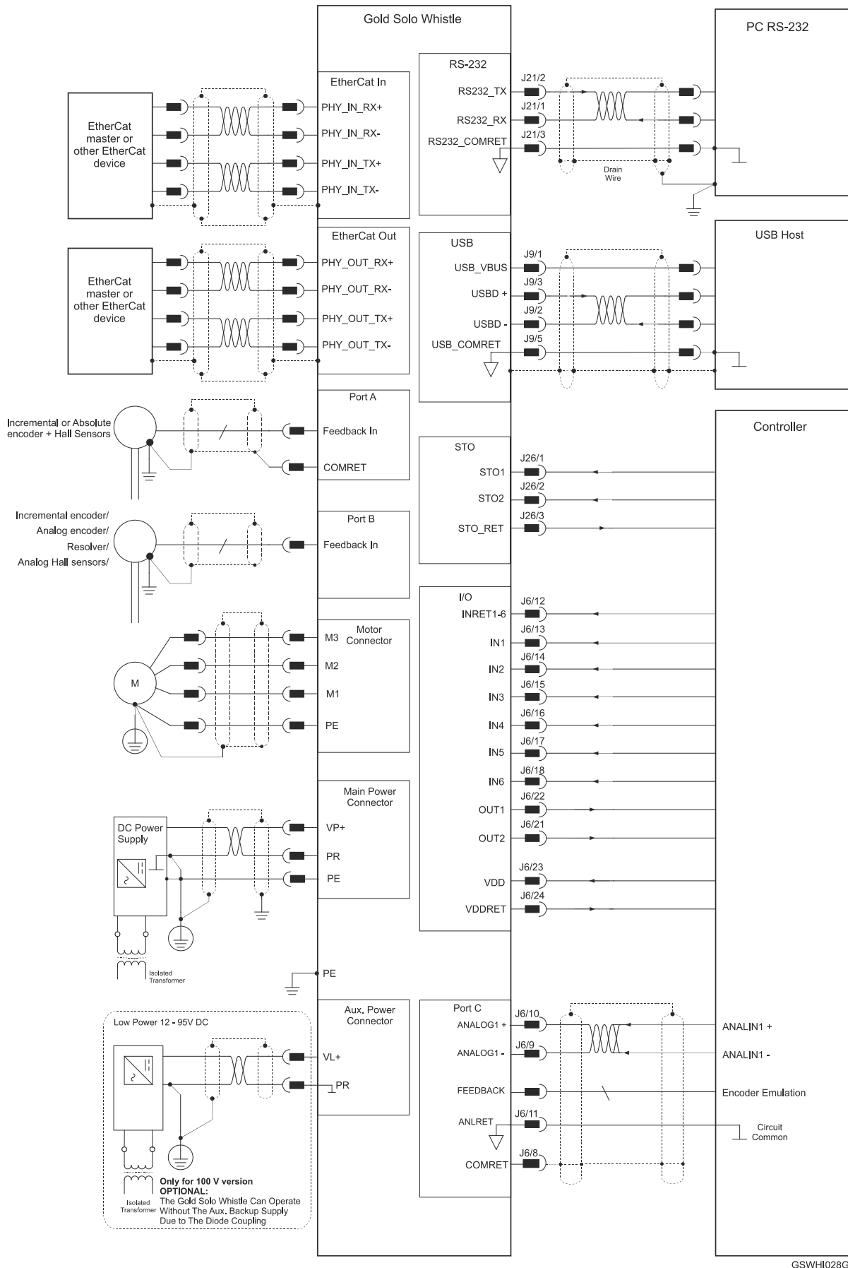
Figure 5: The Gold Solo Whistle Connection Diagram - EtherCAT
