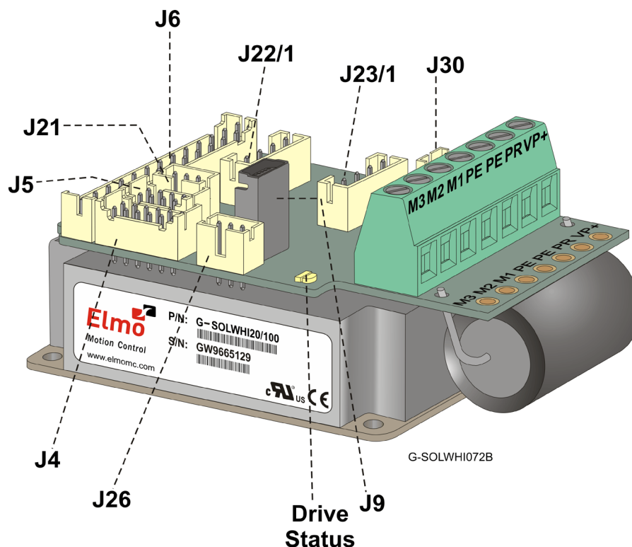
Figure 2: Connector Locations – CAN
